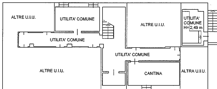
PIANO SEMINTERRATO H= 2,14 m
