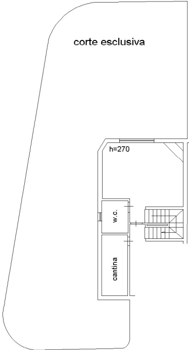
PIANO SEMINTERRATO
